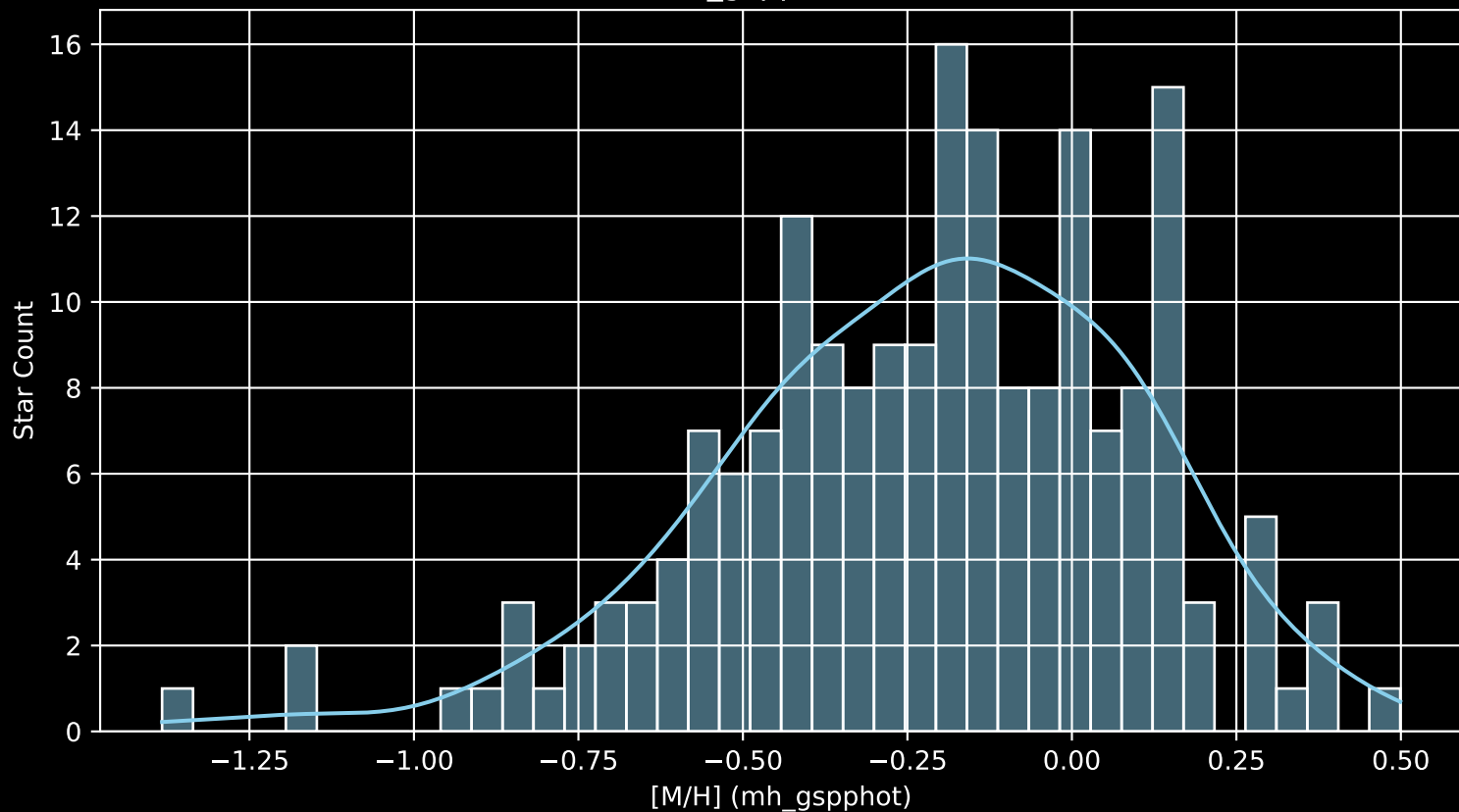
APOGEE DR17 Field: [150+65_MGA [M/H] (mh_gspphot) (n= 191)
