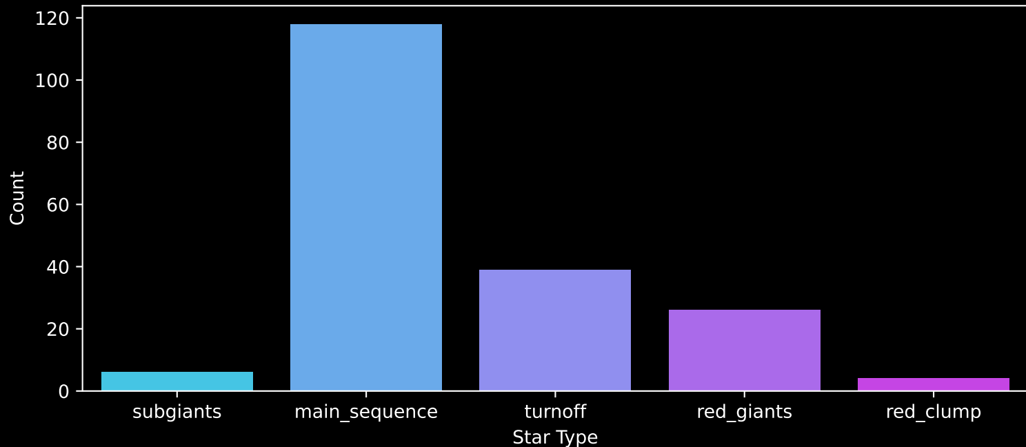
APOGEE DR17 Field: [150+65_MGA] Count plot of Star Type
