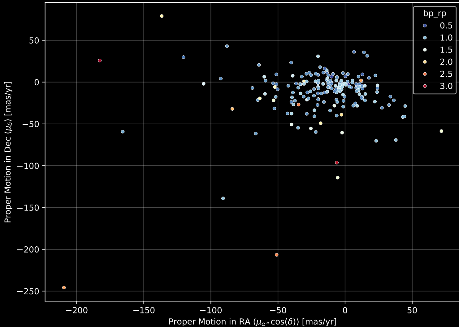
APOGEE DR17 Field: [150+65_MGA] Proper Motion Diagram (n= 193)
