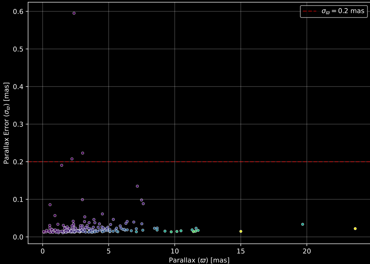
APOGEE DR17 Field: [150+65_MGA] Parallax Quality (n= 193)
