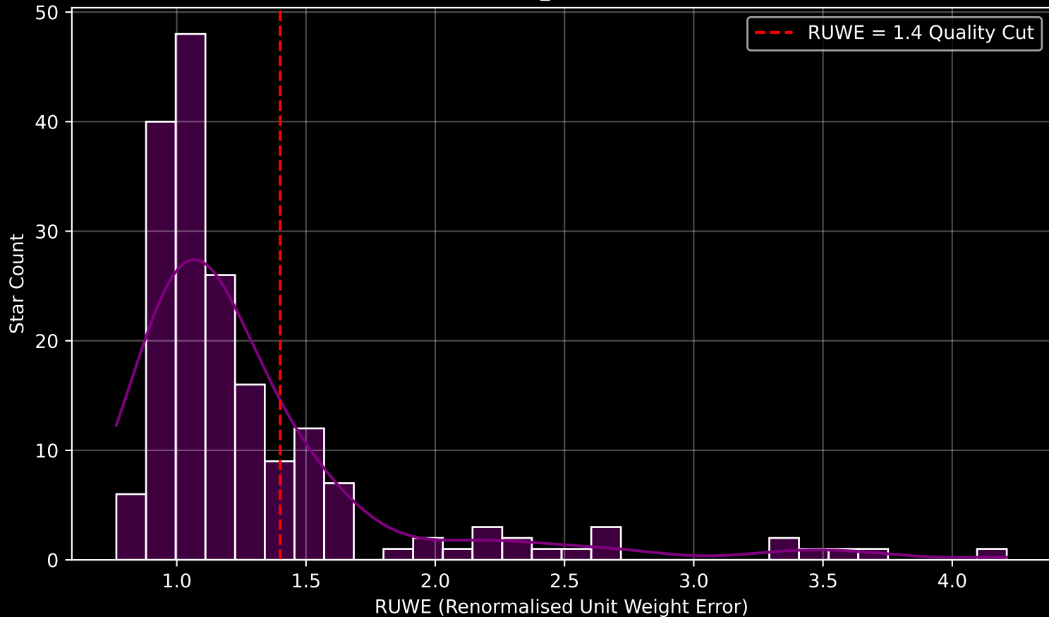
GAPOGEE DR17 Field [150+65_MGA] RUWE Distribution (n= 184)
