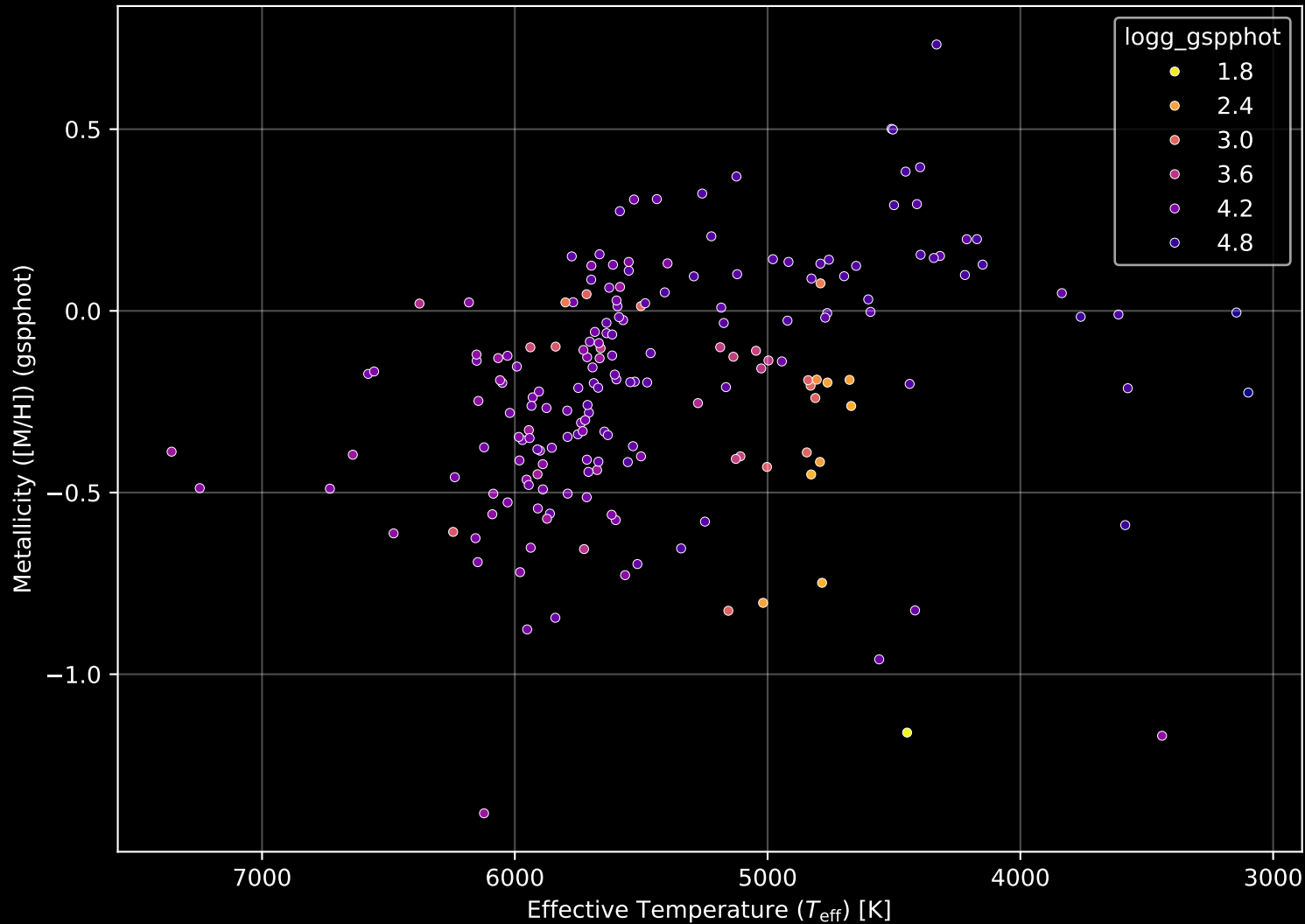
APOGEE DR17 Field: [150+65_MGA] Stellar Population Parameters (n= 193)
